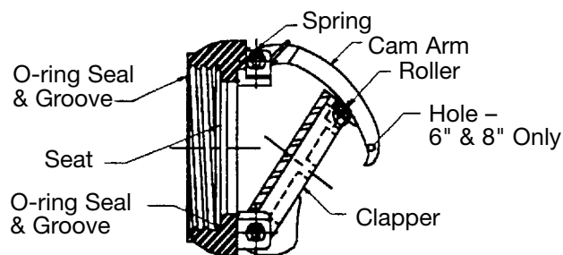
#1 Cam-Check 2 1/2" – 6"
