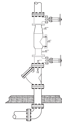
Vertical Installation
