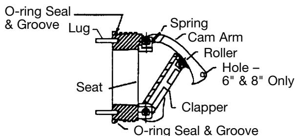
#2 Cam-Check DC & RP
